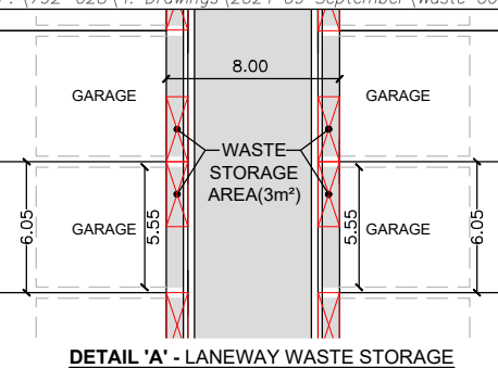
DETAIL 'A' - LANEWAY WASTE STORAGE
