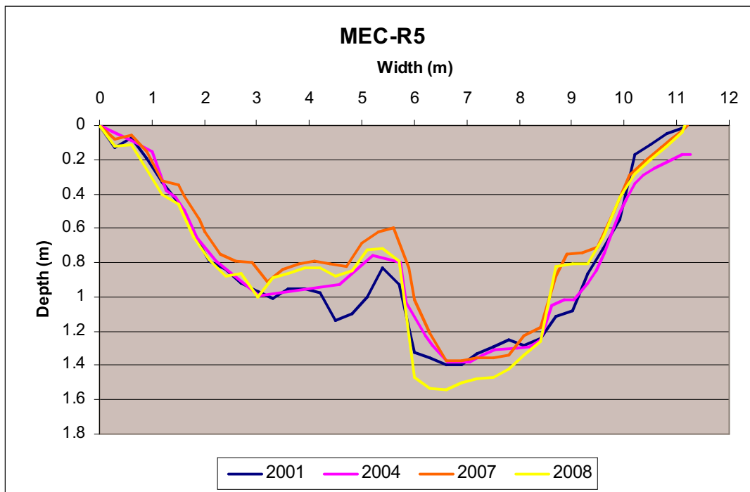
Figure 4.4.3: Cross-sectional monitoring results from 2001-2008 for Site MEC-R5.
