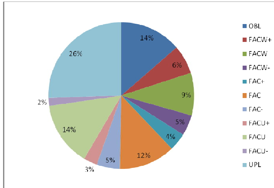
Figure 4.7.1. Ecological spectrum of the flora of the study area: wetness index - OBL, FACW+, FACW, FACW-, FAC+, FAC-, FACU+, FACU, FACU-, UPL (see Appendix H-3 for species ratings).
