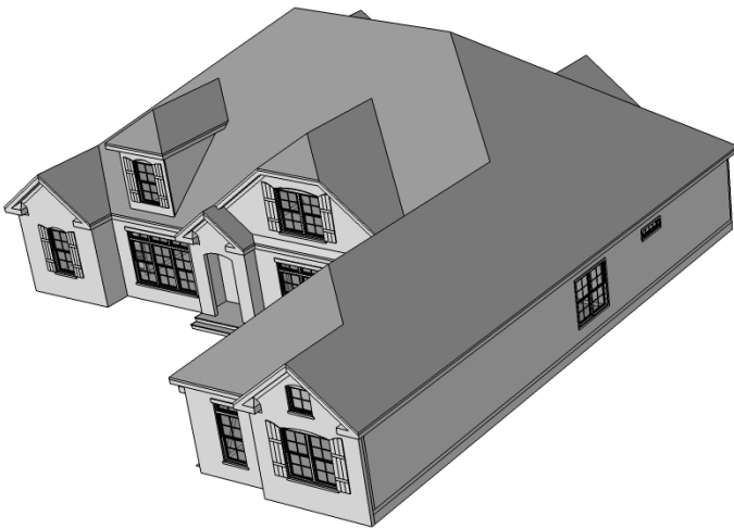
Figure 40: Proposed Model
