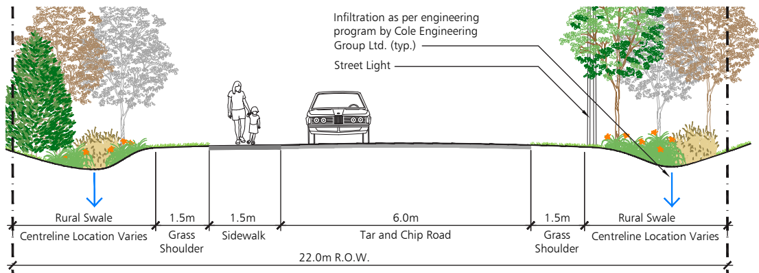
Figure 32: Typical Rural Swale Section on 22m ROW
