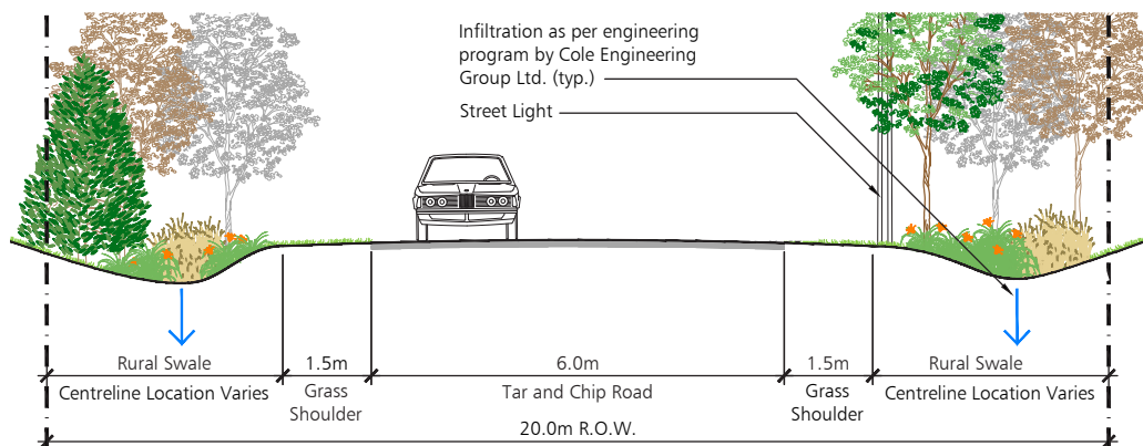
Figure 33: Typical Rural Swale Section on 20m ROW
