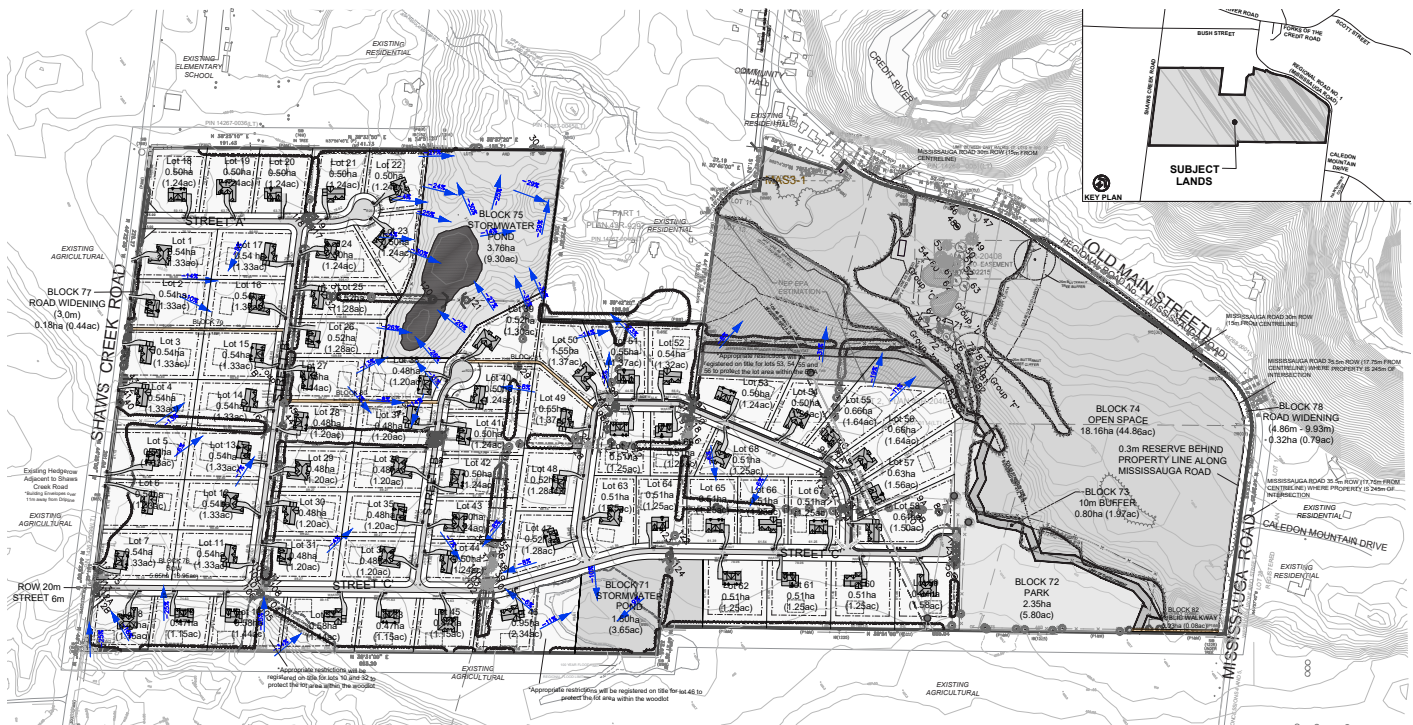
Figure 26: Development Concept Plan with slopes.
