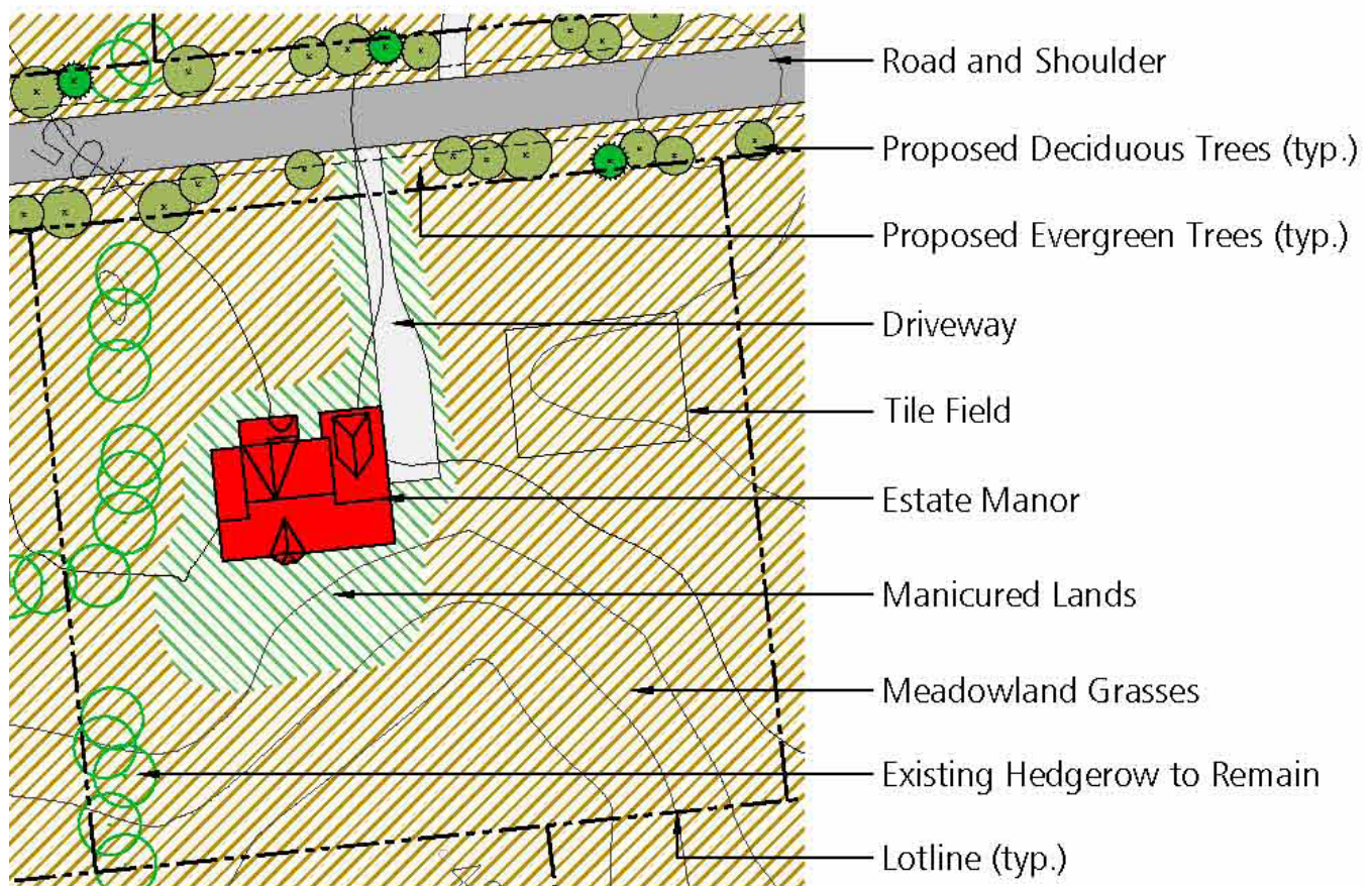
Figure 27: Proposed Site Design, Typical
