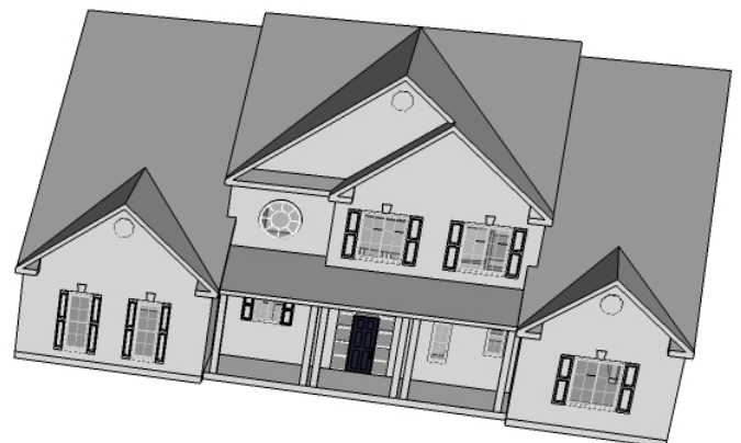
Figure 43: Proposed Model
