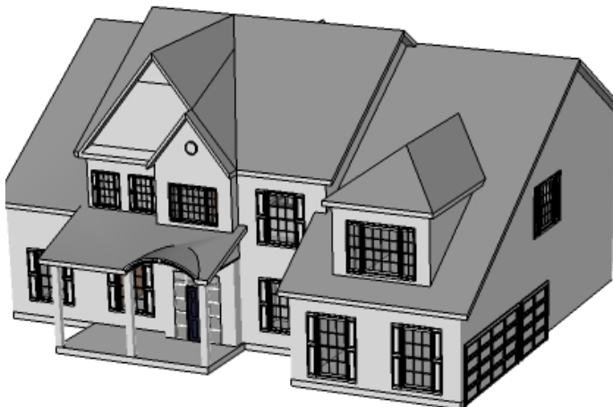
Figure 42: Proposed Model
